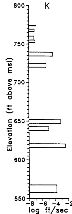
NOTE 1—Elevation is on the vertical axis (land surface is 800 ft (243.84 m) above msl), thickness of bar indicates length of open interval, length of the bar indicates measured hydraulic conductivity. Hydraulic conductivity values range over five orders of magnitude (compiled from data in Ref (17)).
