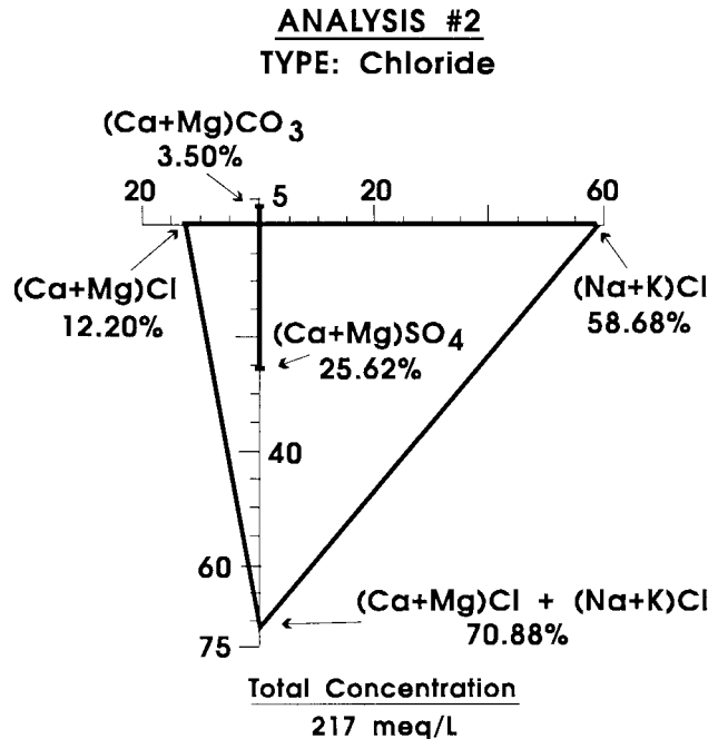
SCALE OF DIAGRAMS IN MEQ/L PERCENTAGE UNITS
