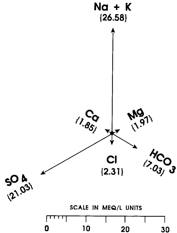
NOTE 1—Adapted from Ref (24). Analysis selected from Ref (1). FIG. 12 Maucha Six-Vector Radial Diagram
