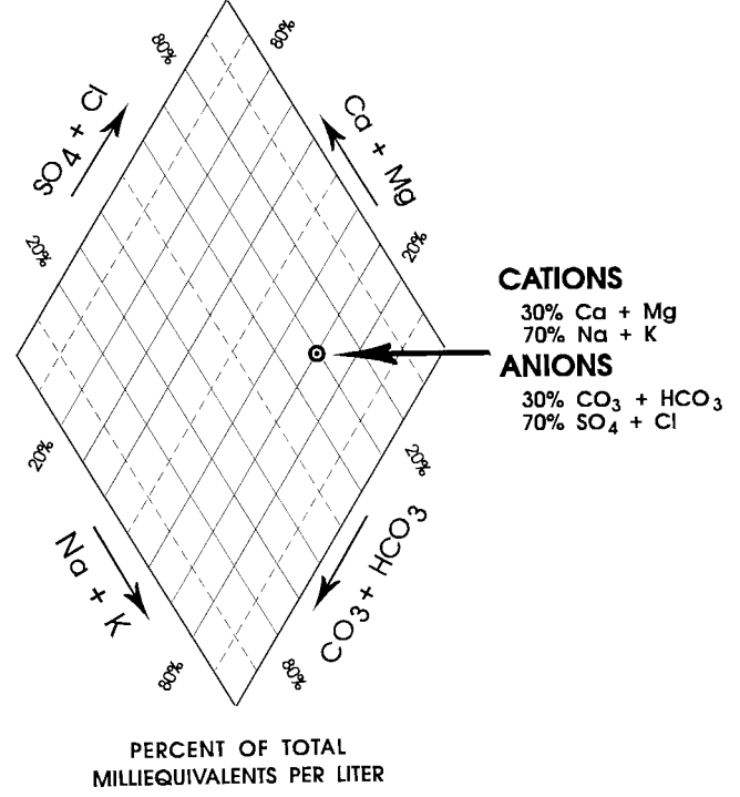
FIG. 10 Example of Diamond Diagram (Adapted from Refs (5) and (6))
