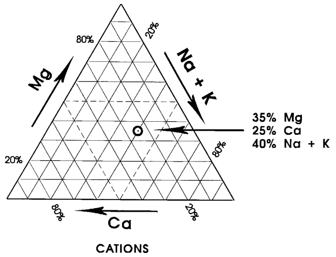
FIG. 9 Example of Trilinear Plot (Adapted from Refs (5) and (6))
