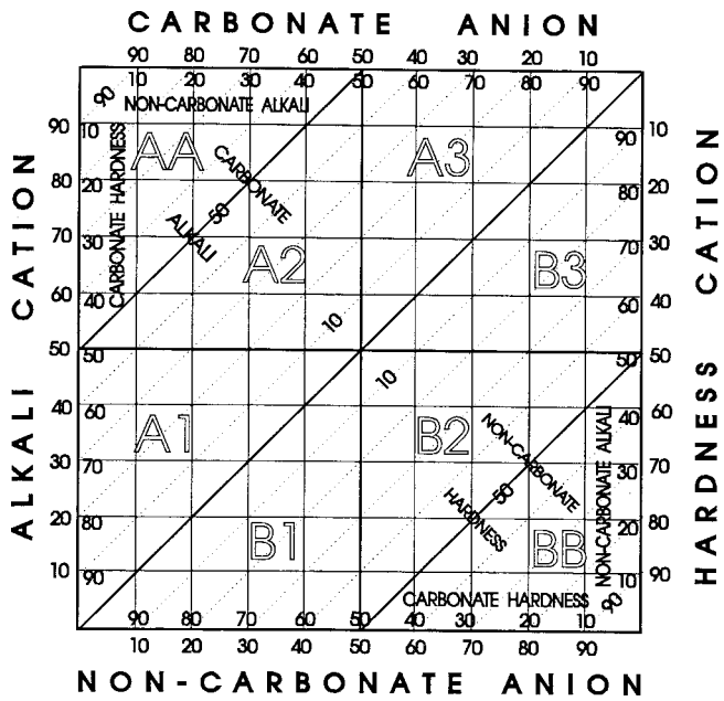
PERCENT OF TOTAL MILLIGRAM EQUIVALENTS PER LITER FIG. 2 Water Classification Diagram (Adapted from Ref (4))
