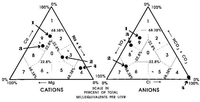
FIG. 7 D'Amore, et al Classification Diagram (see Table 4 for Plotted Parameters)
