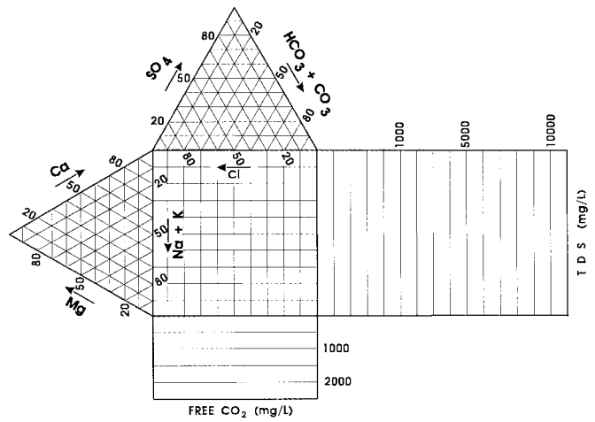
FIG. 4 Water Classification Diagram (Adapted from Ref (7))
