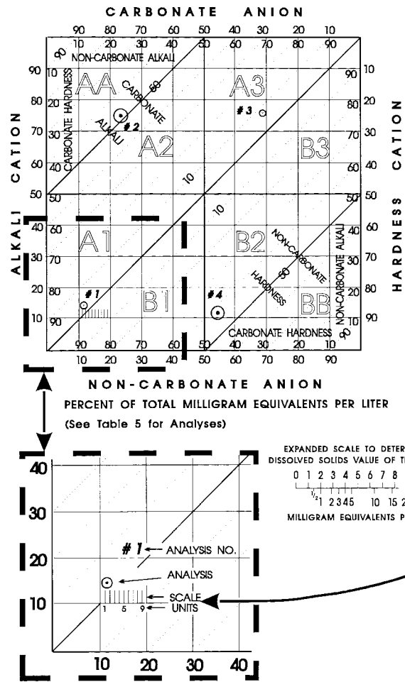
FIG. 13 Example of Water Classification Diagram (Adapted from Ref (4))
