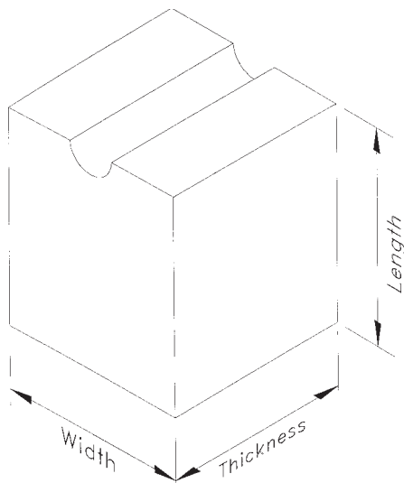
FIG. 1 Specimen Configuration
