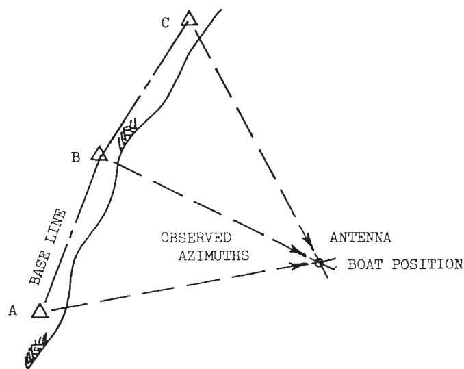
FIG. 9 Triangulation/Intersection
