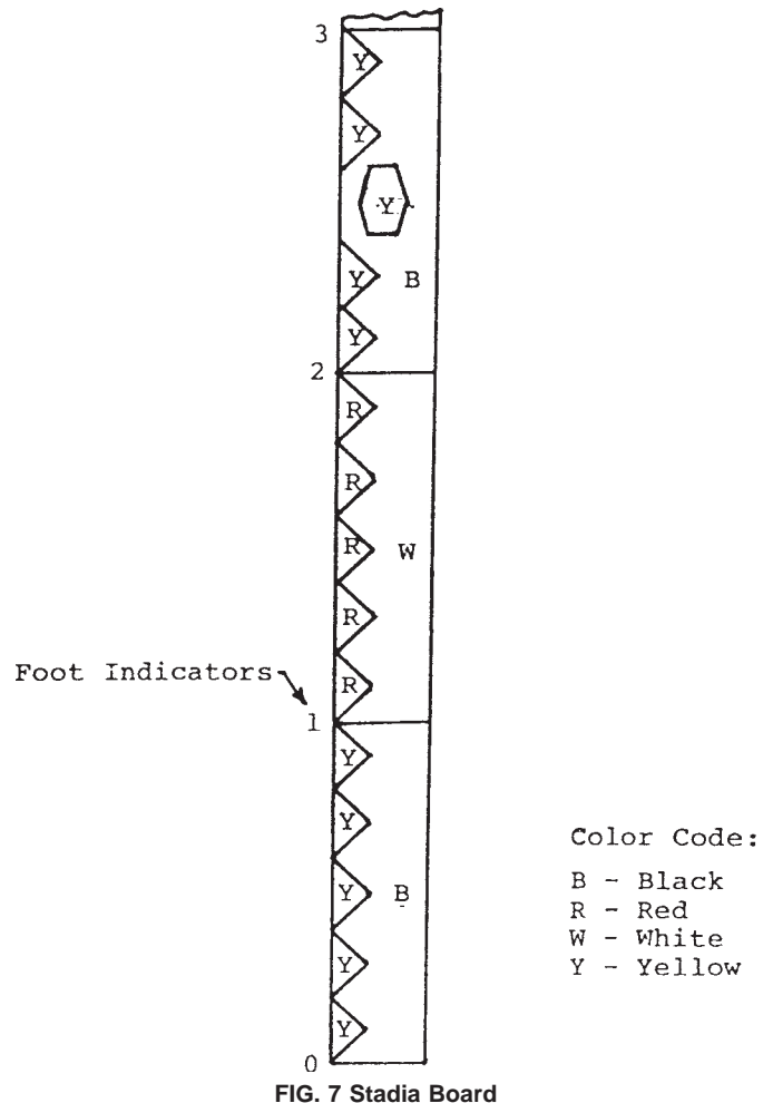
FIG. 7 Stadia Board
