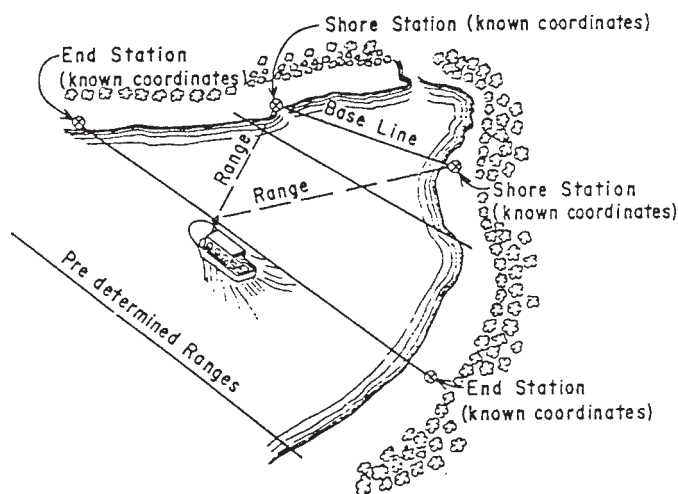
FIG. 13 Range-Range Tracking
