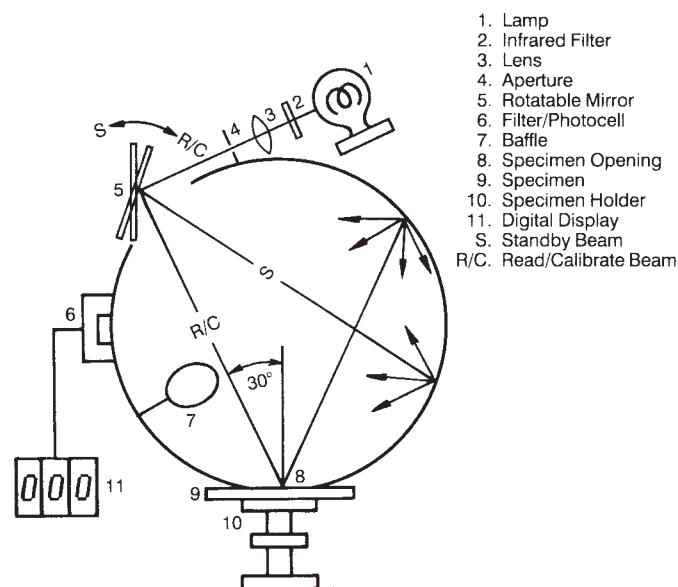
FIG. 1 Schematic Diagram of Reflectometer
